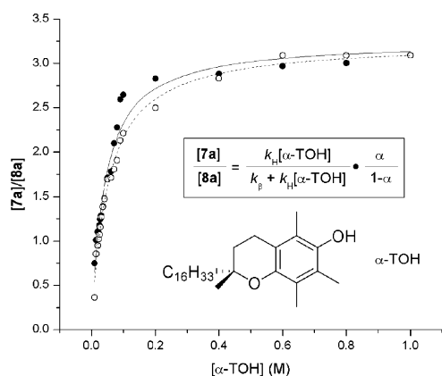
Fig. 1 Ratio of 7a to 8a formed from the decomposition of 9 as a function of [\alpha\text{-TOH}] following 4 h at 37 °C in benzene (●, —) and following 30 min irradiation (300 nm) at 25 °C in benzene (○, - -).
